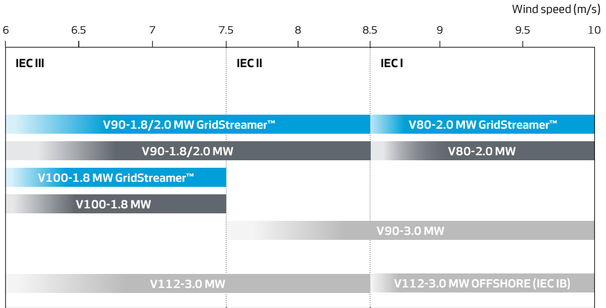
Fig 1. Overview of Vestas wind turbines operating in the various wind classes
